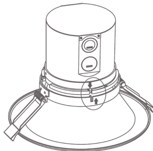
Align and Twist-lock Light Engine with Trim
