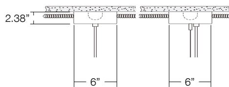
CY-4H 6" Surface Canopy for Power Cable (Covers 40 Box)
