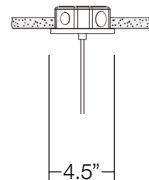
CY-4H 4" Canopy with Power Cable (Covers 40 Box)
