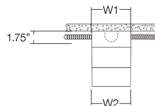
CY-6H 6" Surface Canopy (Covers 40 Box)
