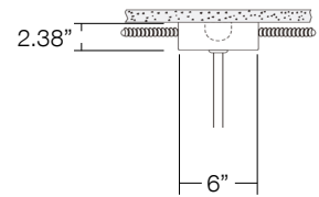
CY-4H / CY-6H 6" Surface Canopy for Stem Mount (Covers 40 Box)
