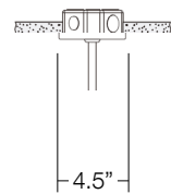
CY-4H / CY-6H 4" Canopy for Stem Mount (Covers 40 Box)
