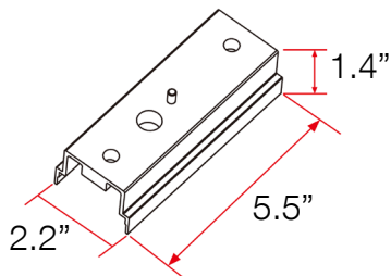
LX2.3-CON LUX 2.3" Profile Line Joiner (metal bracket)
