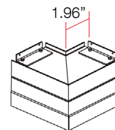
LX3.8P-CON-OUT LUX 3.8" Perimeter 90° Illuminated Outside Corner
