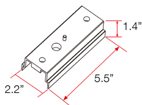
LX3.8-CON LUX 3.8" Profile Line Joiner (metal bracket)
