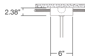
CY-4H / CY-6H 6" Surface Canopy for Stem Mount (Covers 40 Box)
