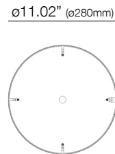
11" Surface Mount Canopy
