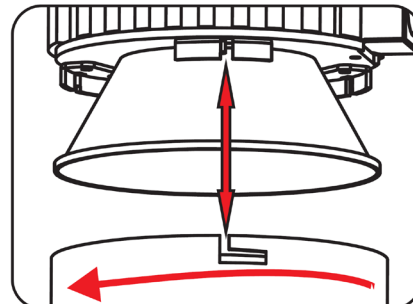
Line up trim and engine, turn clockwise to lock
