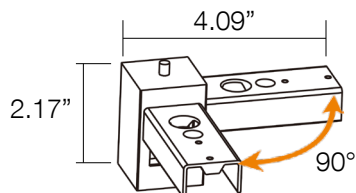
LX1.3-CON-N-L LUX 1.3" Profile "L" 90DEG NonLit Corner
