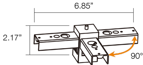
LX1.3-CON-N-T LUX 1.3" Profile "T" 90DEG NonLit Corner
