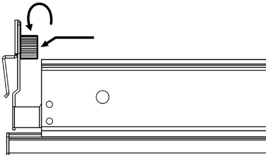
Loosen T-Grid clip locknuts (both ends)
