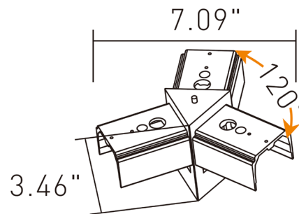
LX2.3-CON-N-Y LUX 2.3" Profile "Y" 120DEG NonLit Corner (metal bracket)
