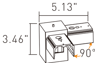
LX2.3-CON-N-T LUX 2.3" Profile "T" 90DEG NonLit Corner (metal bracket)
