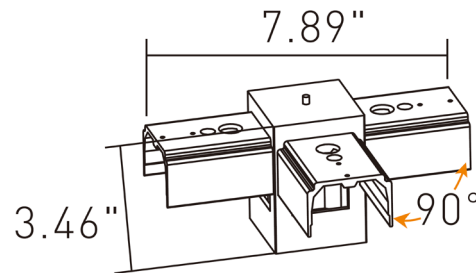
LX2.3-CON-N-T LUX 2.3" Profile "T" 90DEG NonLit Corner (metal bracket)
