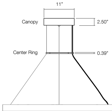
CM2 - Canopy Mount w/ Center Ring
