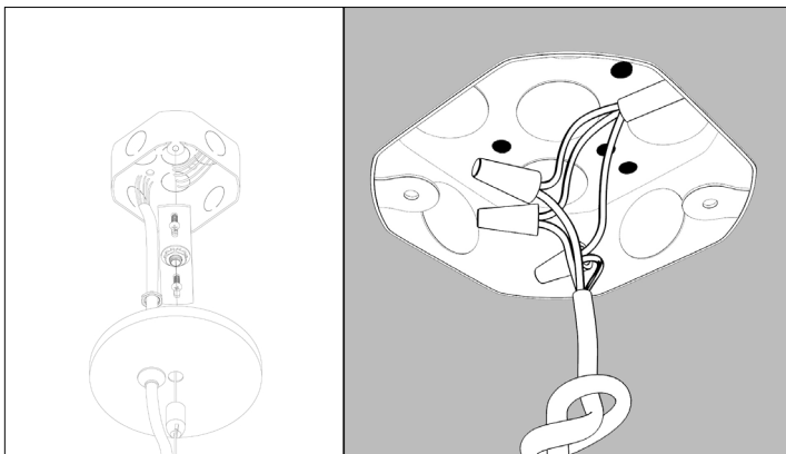
7. Mount canopy bracket to the J-box and make wiring connection. Refer to final/record for reference. Ensure Power is OFF prior to connecting wiring. CAUTION: Do not pinch wire connections.
