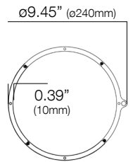
Center Ring w/Single Wire Hole
