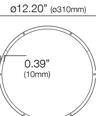
Center Ring w/Double Wire Hole
